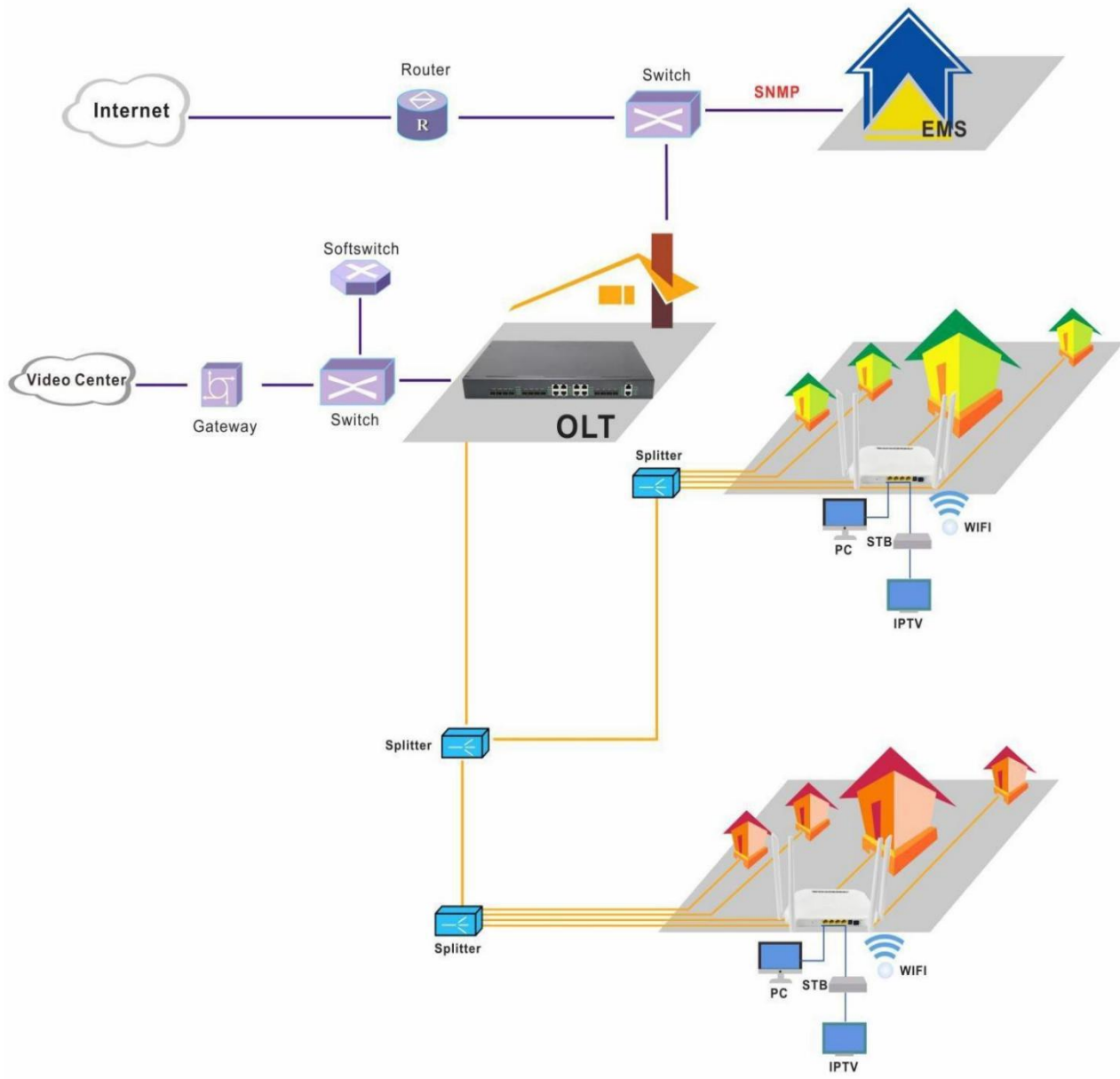
Figure: UW-315VPW Application Diagram
